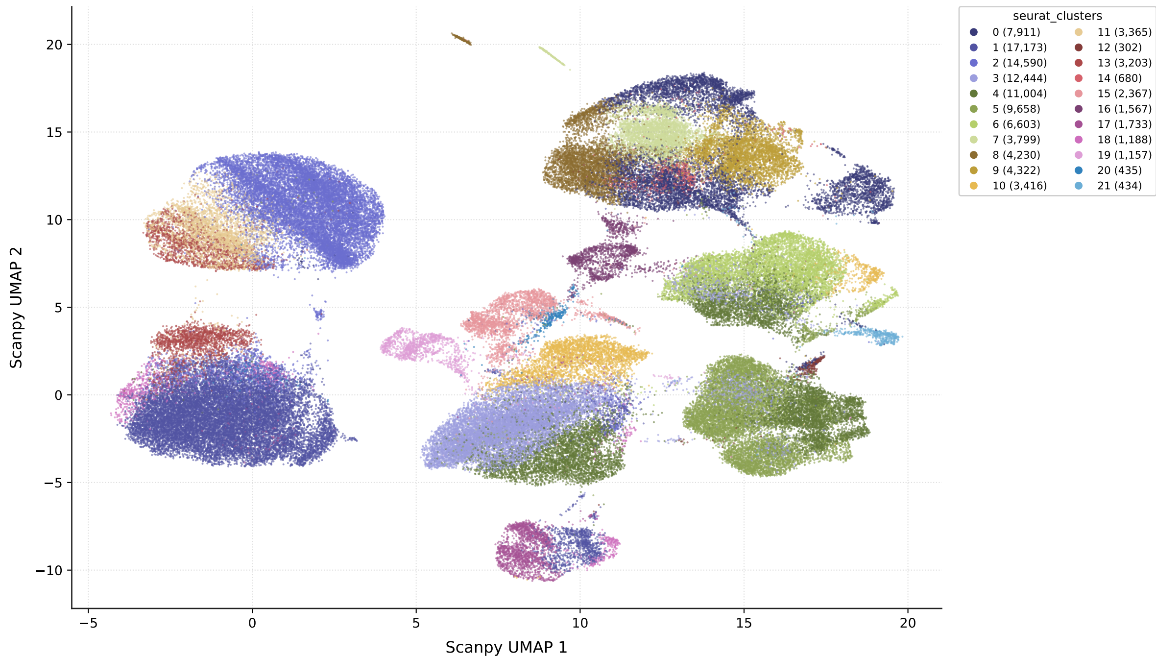
Scanpy UMAP: seurat_clusters (n = 111,581 cells, 22 groups)
