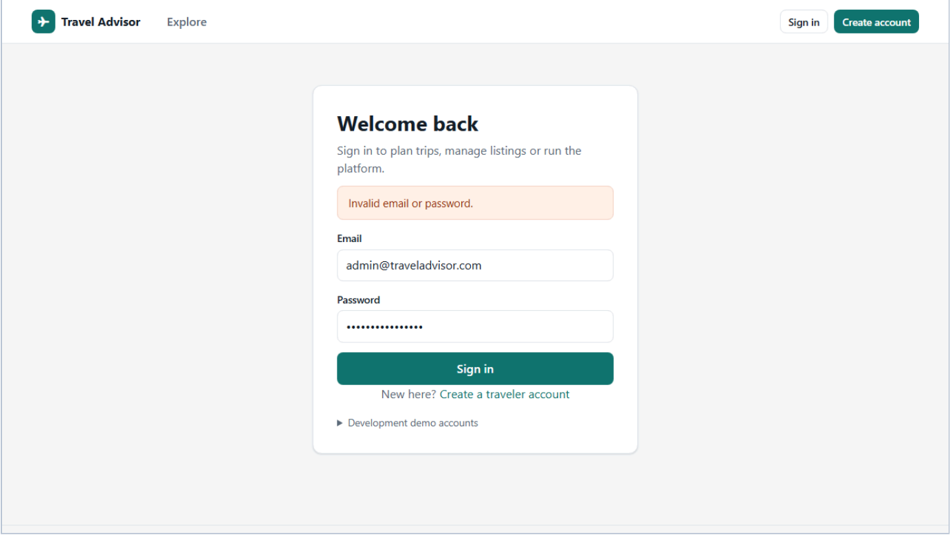
Browser at the end of the test (Playwright screenshot: on).
