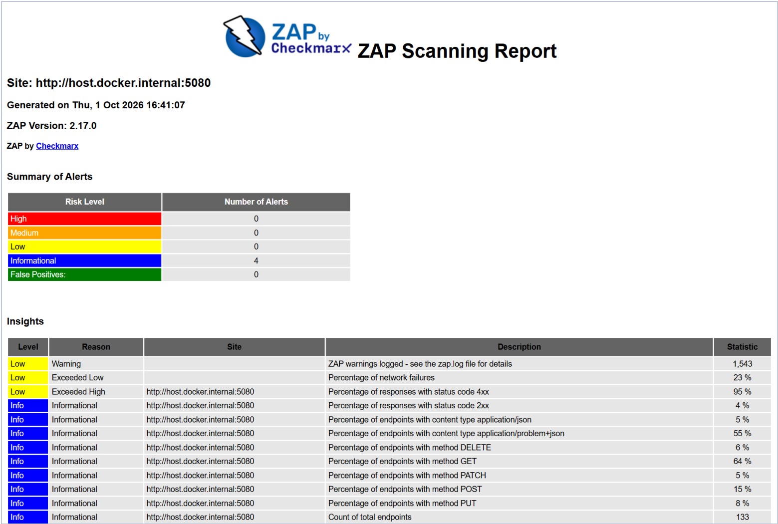
Report of the final api scan (2026-10-01). The Summary of Alerts table counts the alerts per risk level.
