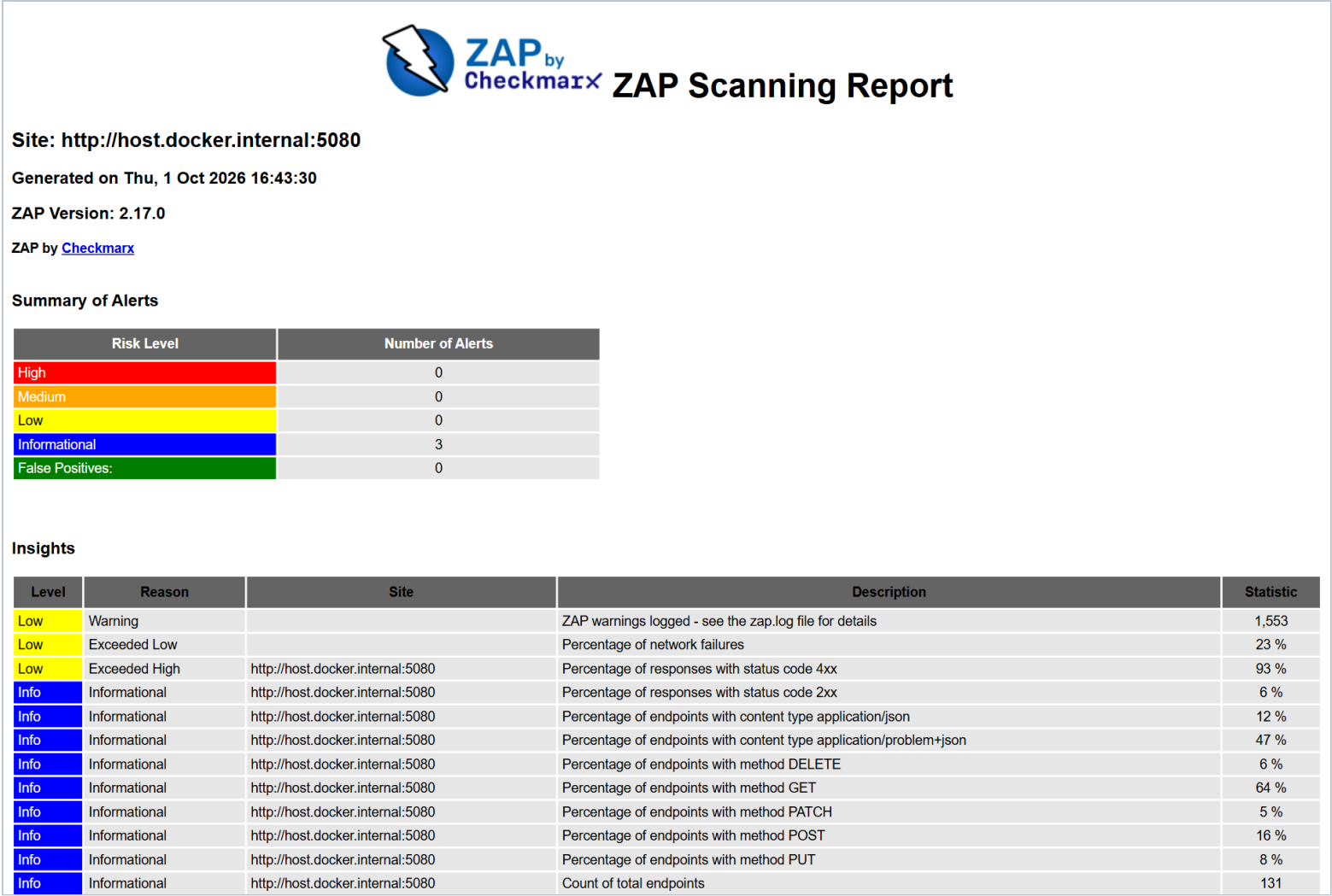
Report of the final api-user scan (2026-10-01). The Summary of Alerts table counts the alerts per risk level.
