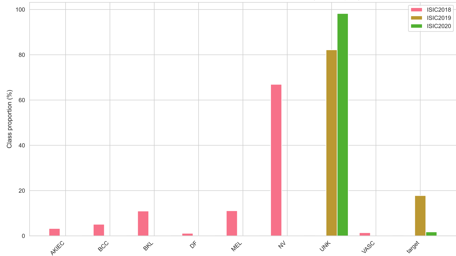
ISIC2018 vs ISIC2019 vs ISIC2020 – label distribution (TRAIN splits)
