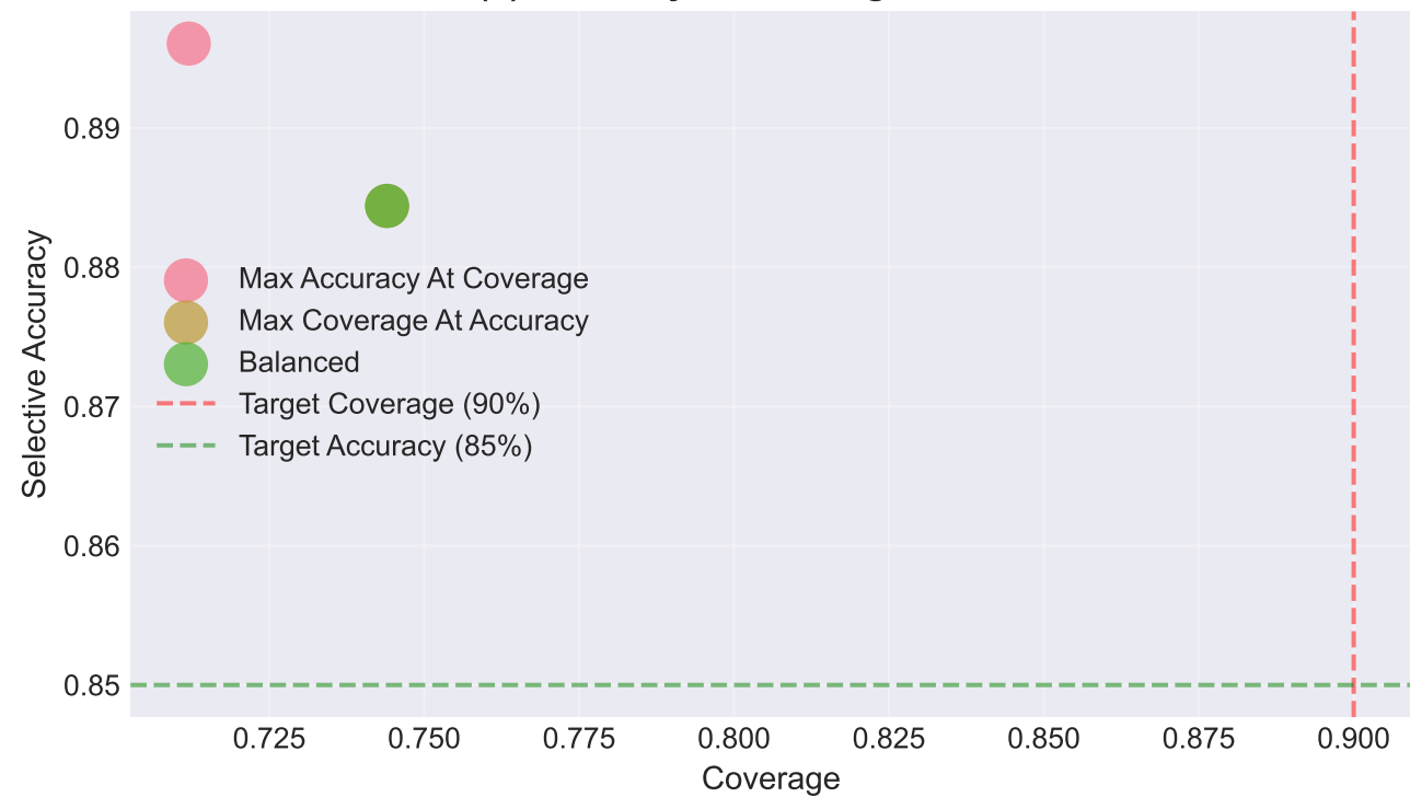
(b) Accuracy vs Coverage Trade-off
