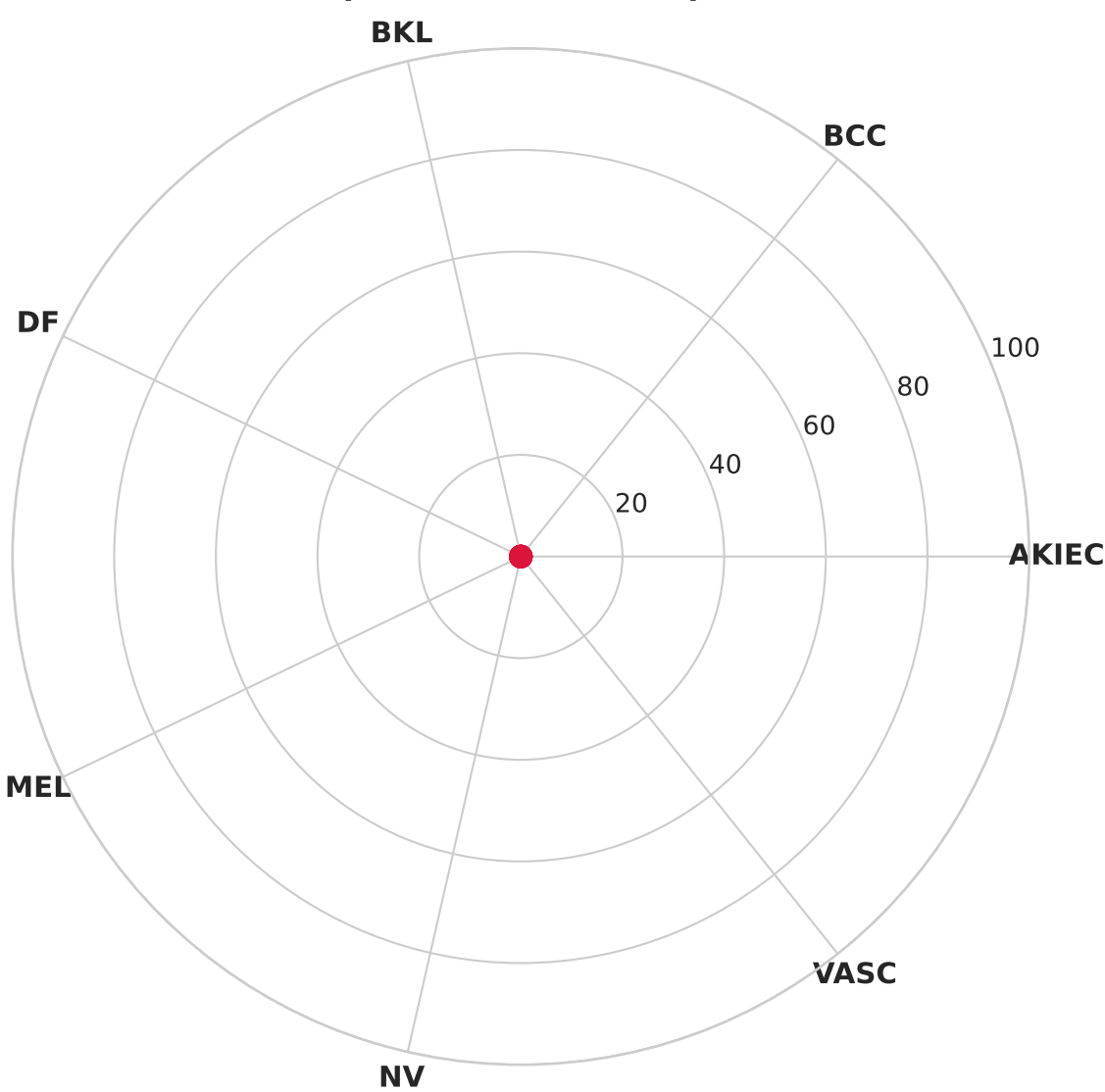
(c) Per-Class Robustness Profile (PGD-40 \epsilon=8/255 )
