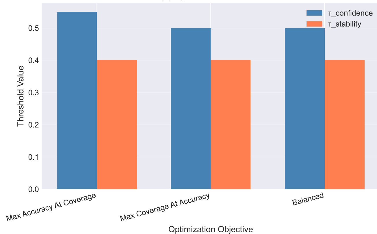
(a) Optimal Thresholds
