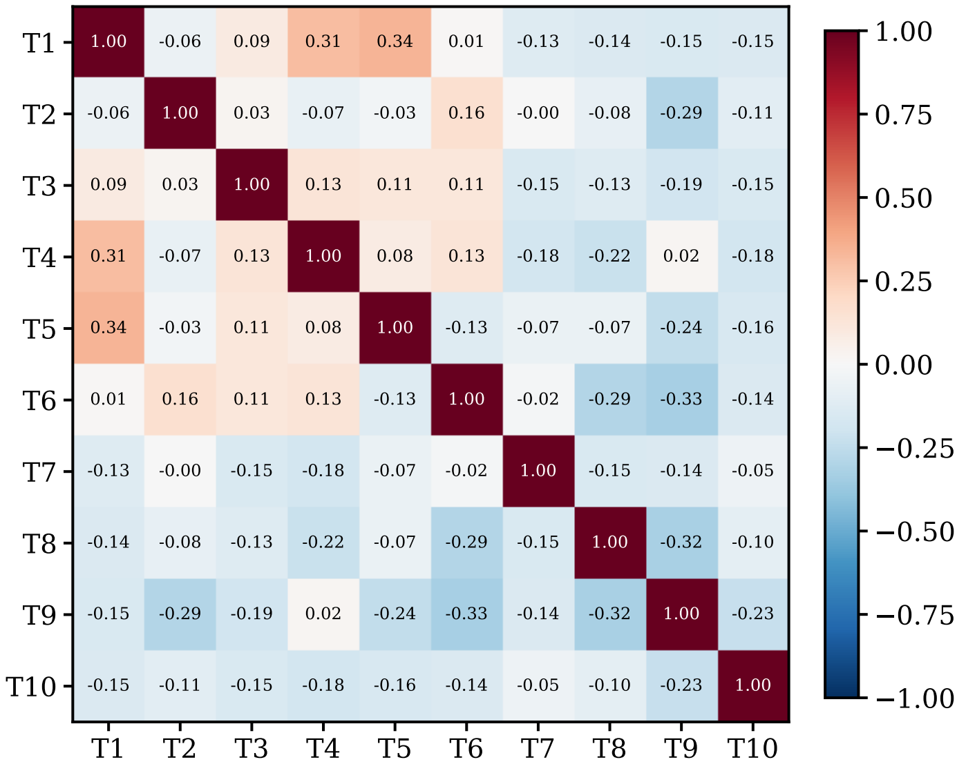
NMF activation coefficient correlations
