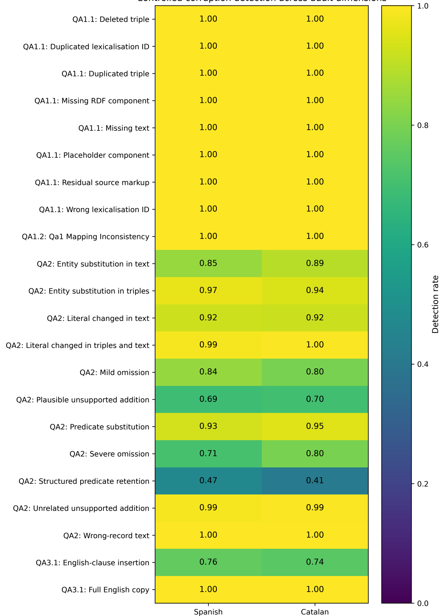
Controlled corruption detection across audit dimensions
