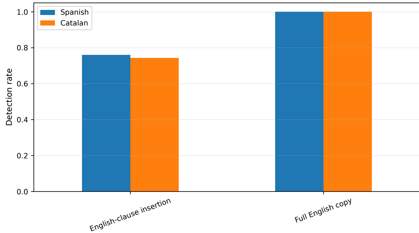
QA3 controlled language-corruption detection
