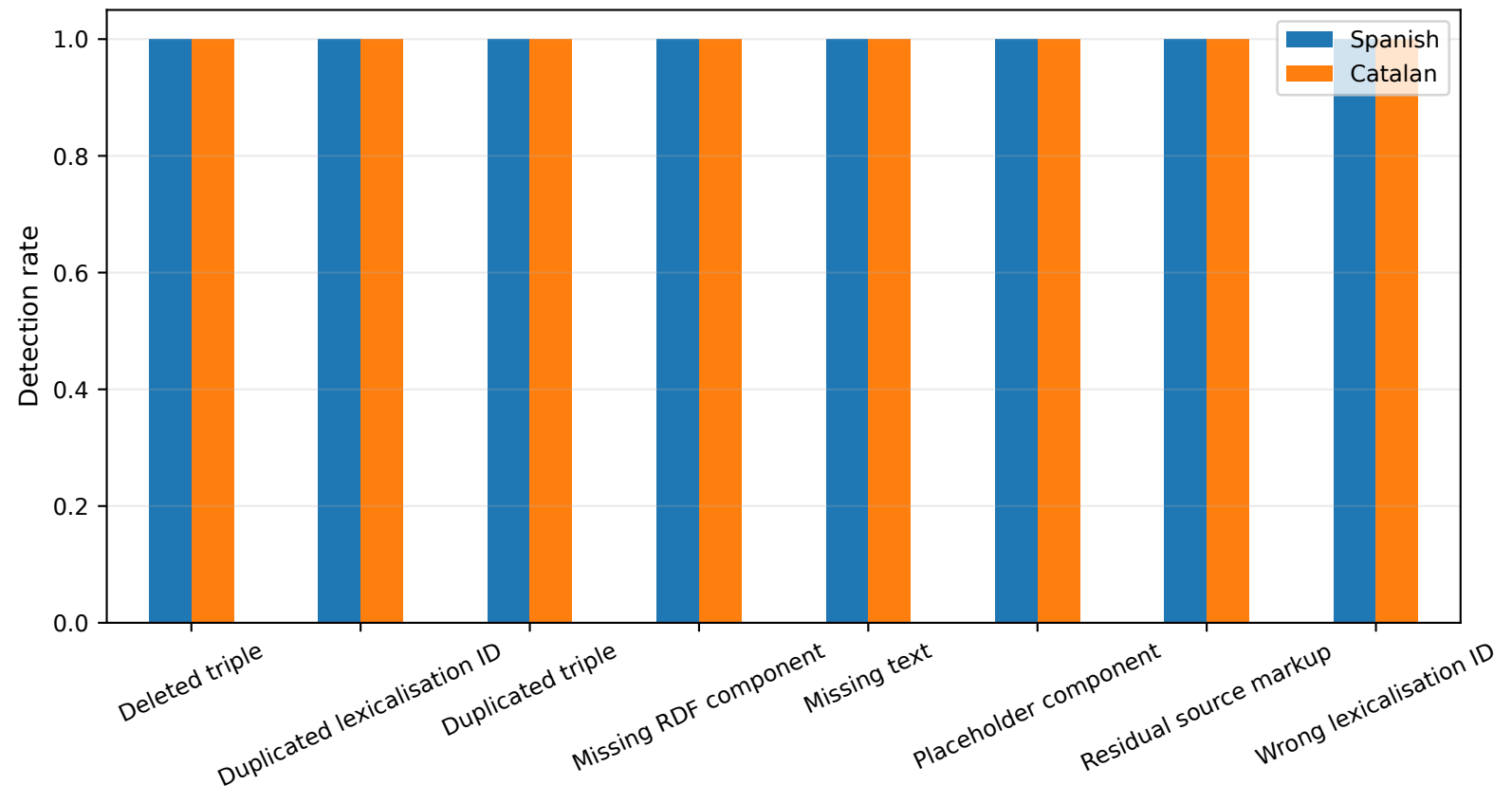
QA1.1 structural-corruption detection
