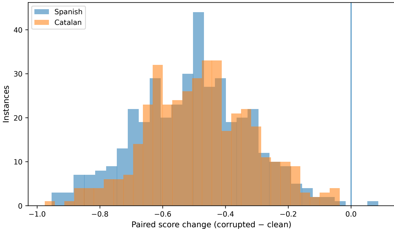
QA2 distribution: Wrong-record text
