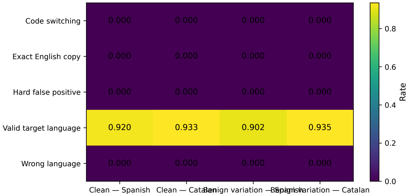
QA3 language-diagnostic false-positive rates on controls
