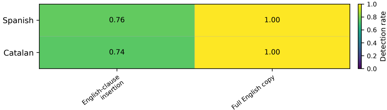
QA3: Target-language corruption detection
