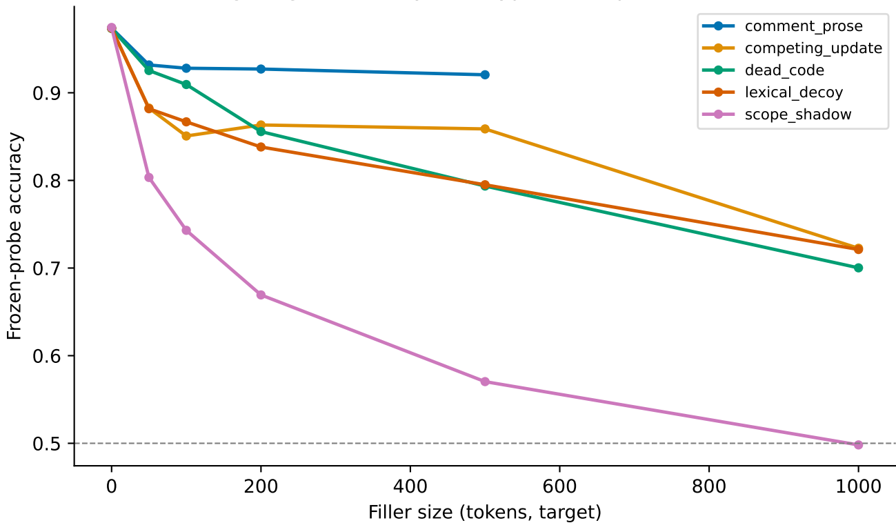
binding: degradation by filler type — deepseek-coder-6.7b
