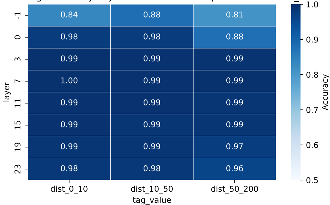
Def-use edge accuracy: layer x distance — deepseek-coder-1.3b_core
