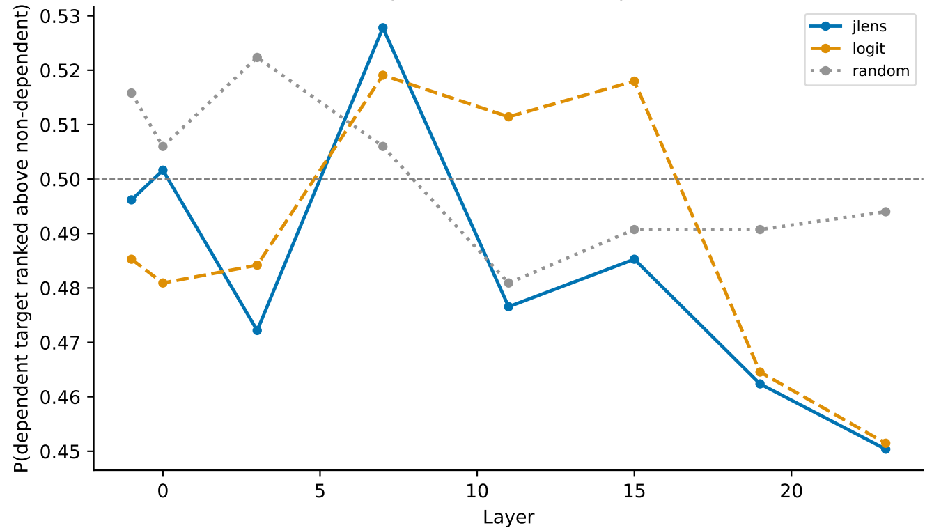
E10-3 control dependence, all — deepseek-coder-1.3b
