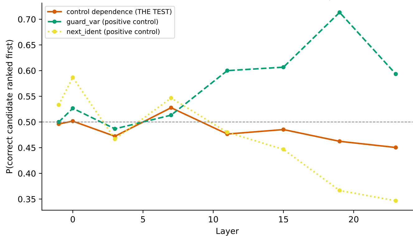
E10-3: is the null a dissociation or a dead readout? — deepseek-coder-1.3b
