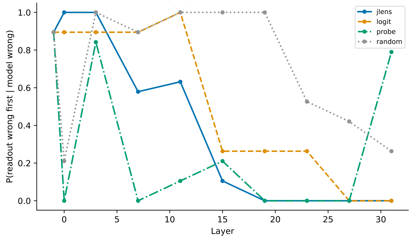
E10-2 early warning by layer and readout — deepseek-coder-6.7b
