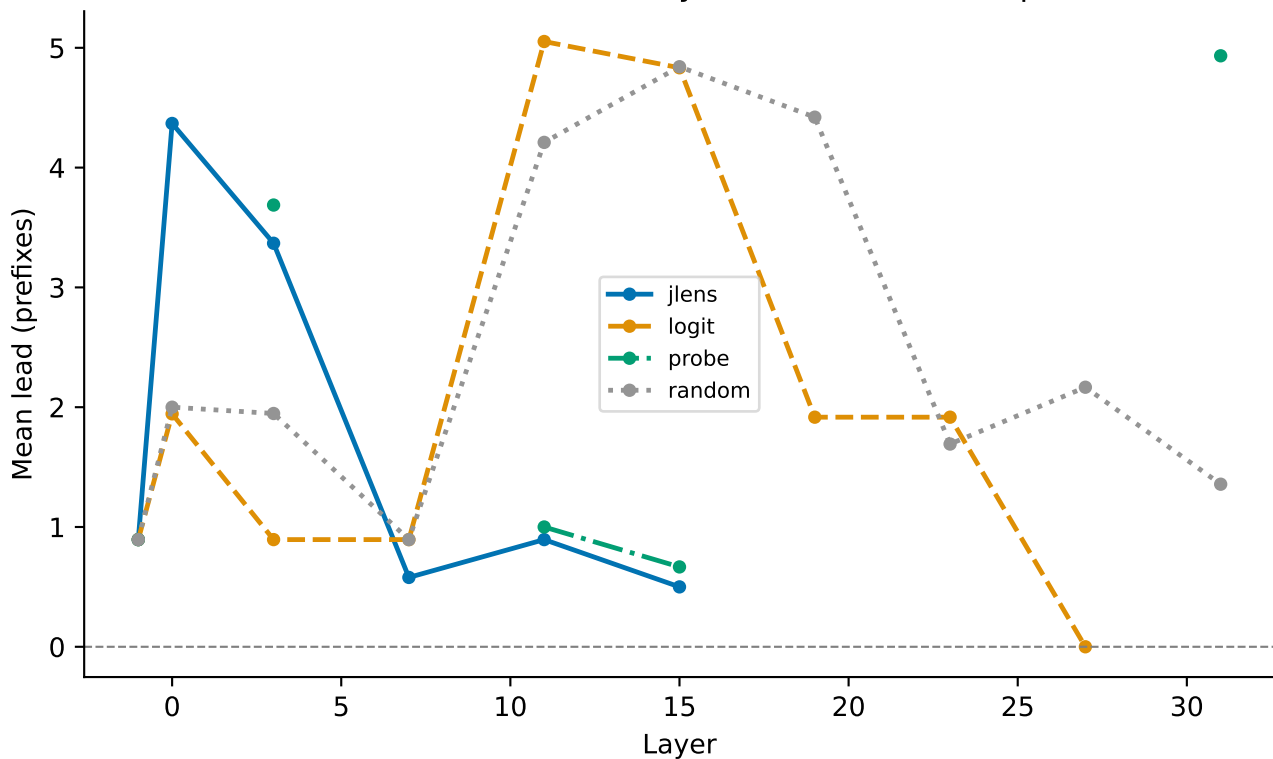
E10-2 mean lead by layer and readout — deepseek-coder-6.7b (denominator moves across layers — read the rate plot first)
