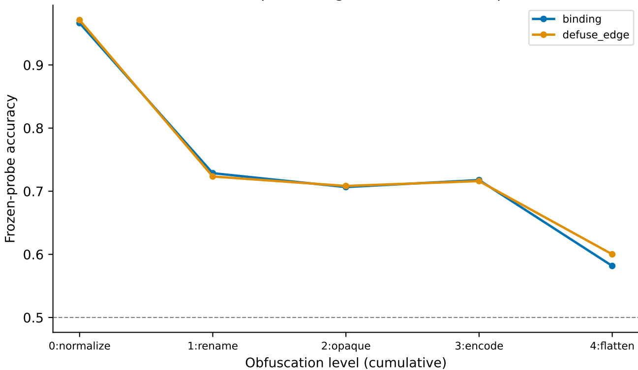
Robustness to semantics-preserving obfuscation — deepseek-coder-1.3b
