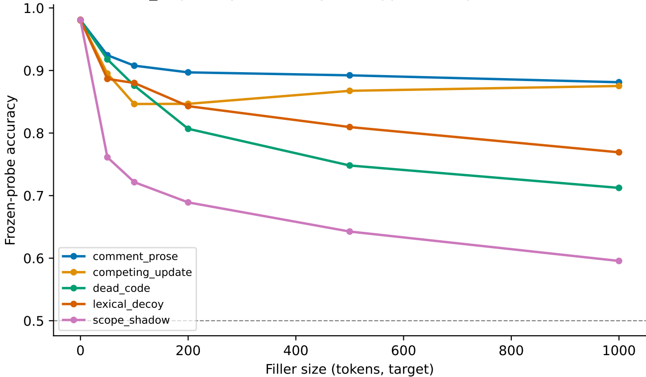
defuse_edge: degradation by filler type — deepseek-coder-6.7b
