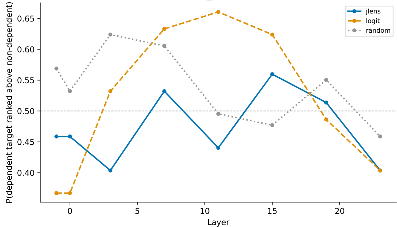
E10-3 control dependence, non_dependent — deepseek-coder-1.3b
