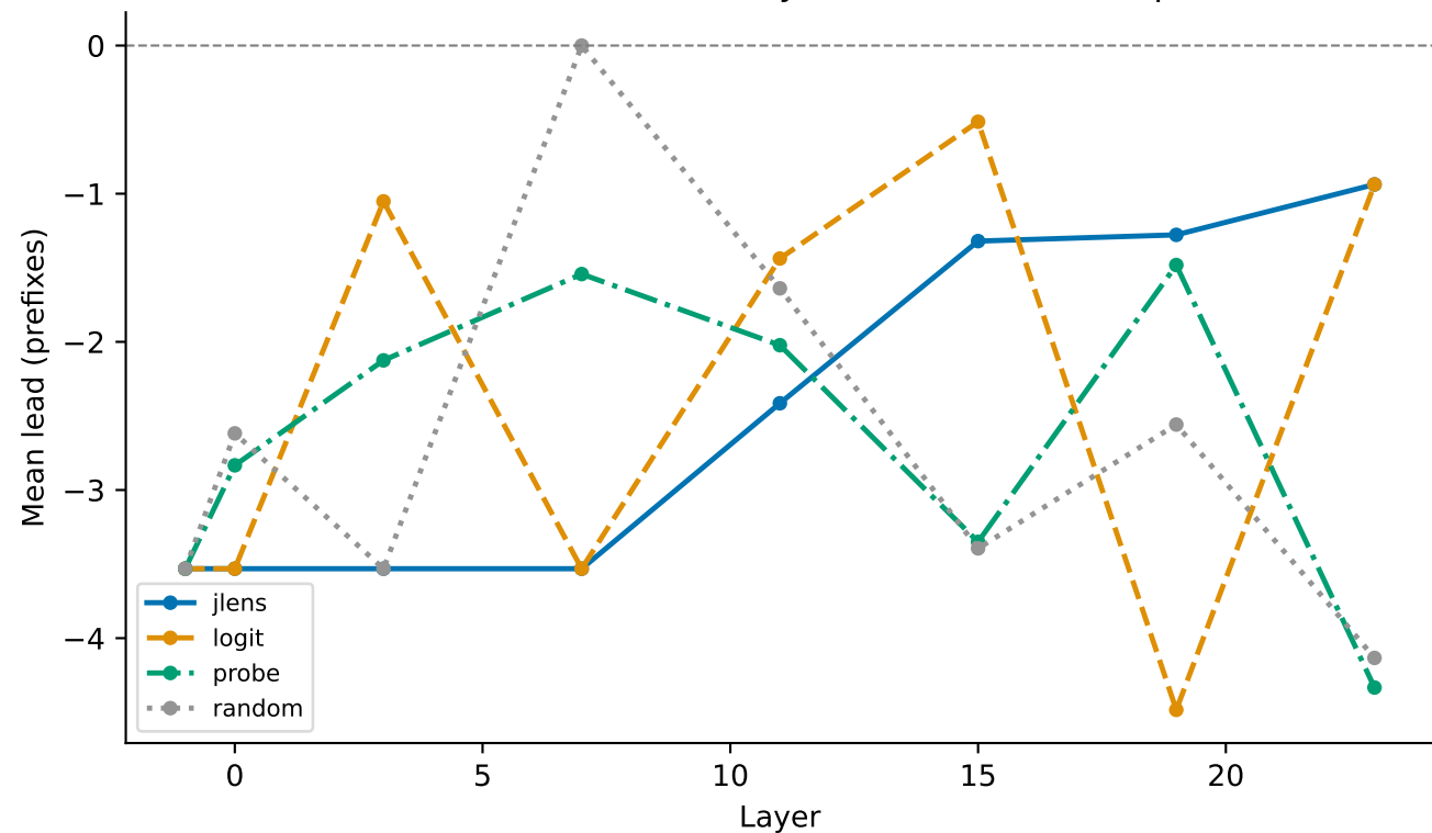
E10-2 mean lead by layer and readout — deepseek-coder-1.3b (denominator moves across layers — read the rate plot first)
