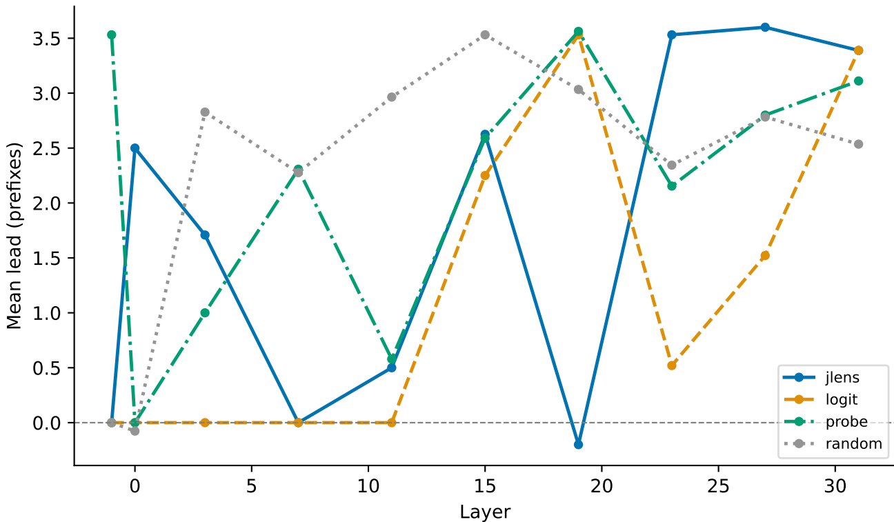
E10-2 mean lead by layer and readout — deepseek-coder-6.7b (denominator moves across layers — read the rate plot first)
