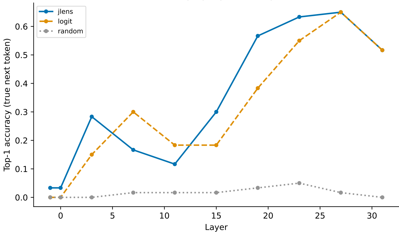
V2 next-token recovery by layer — deepseek-coder-6.7b
