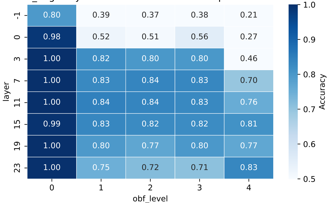
defuse_edge: layer × obfuscation level — deepseek-coder-1.3b
