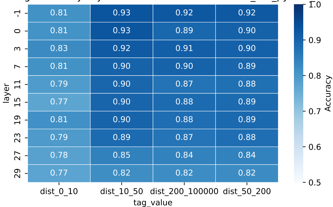
Def-use edge accuracy: layer x distance — starcoder2-3b_csn_python_200
