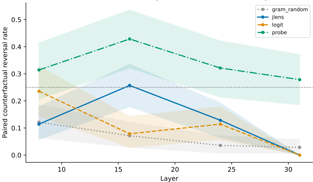
E11: does the readout flip with the binding? — deepseek-coder-6.7b (at the marked use, test split; band = cluster-bootstrap CI)
