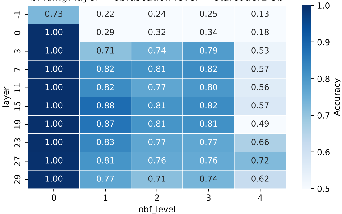
binding: layer x obfuscation level — starcoder2-3b
