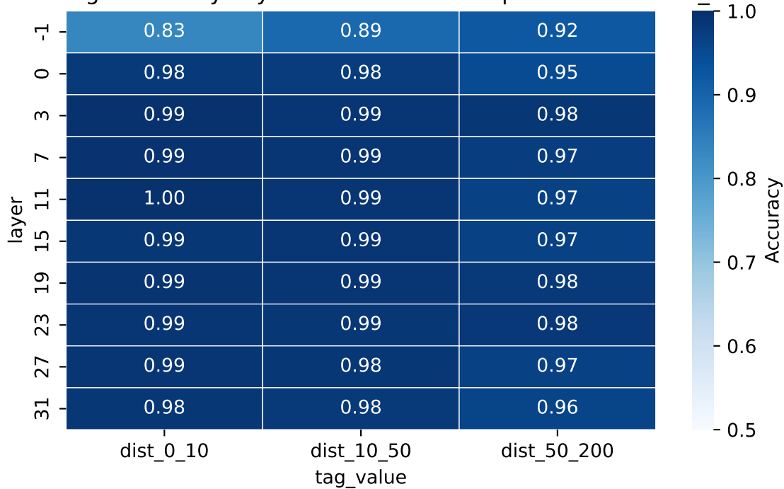
Def-use edge accuracy: layer × distance — deepseek-coder-6.7b_core
