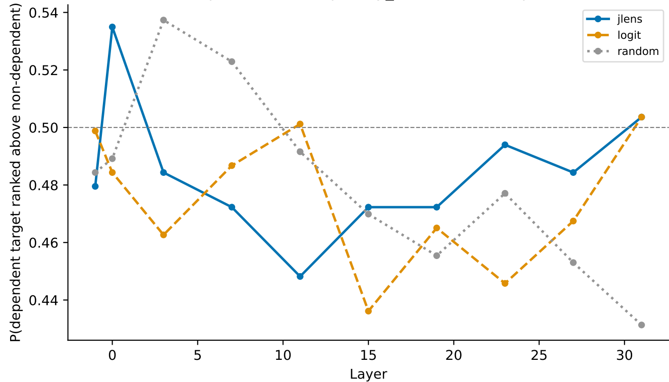
E10-3 control dependence, temporally_matched — deepseek-coder-6.7b
