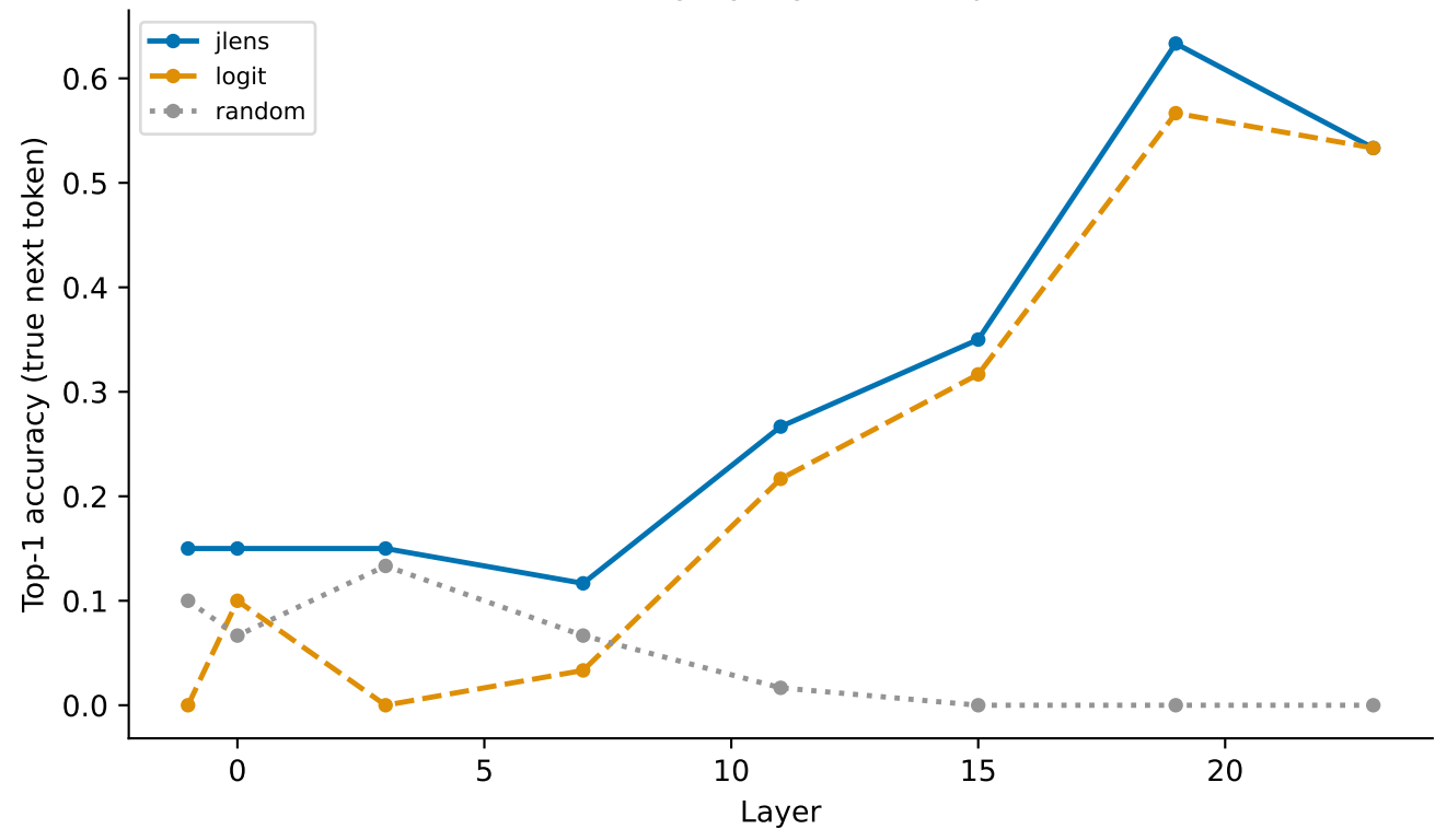
V2 next-token recovery by layer — deepseek-coder-1.3b
