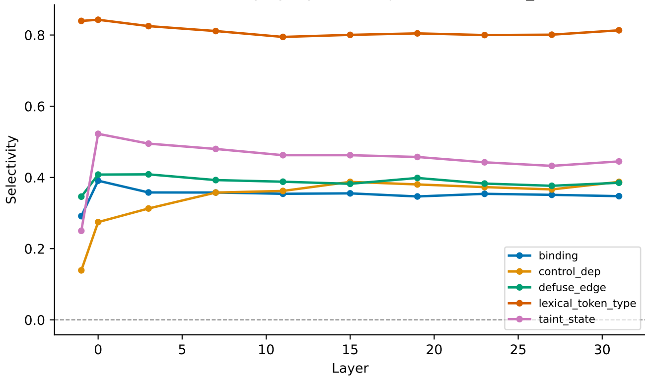
Probe selectivity by layer — deepseek-coder-6.7b_core
