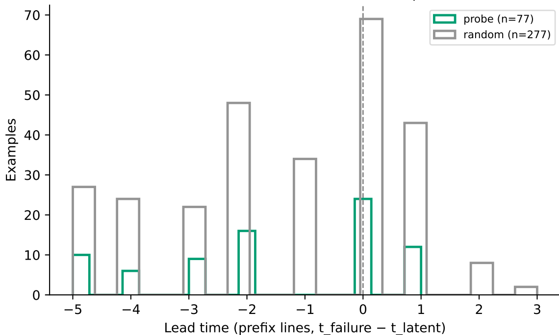
Latent-vs-behavioral failure lead time — deepseek-coder-1.3b
