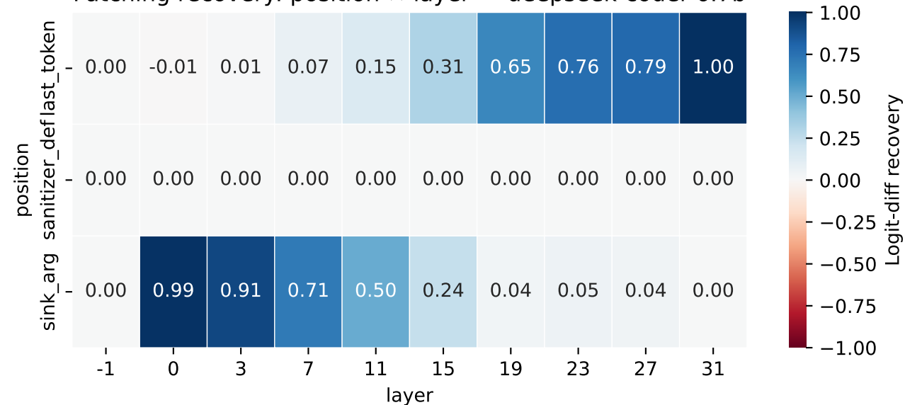
Patching recovery: position \times layer — deepseek-coder-6.7b
