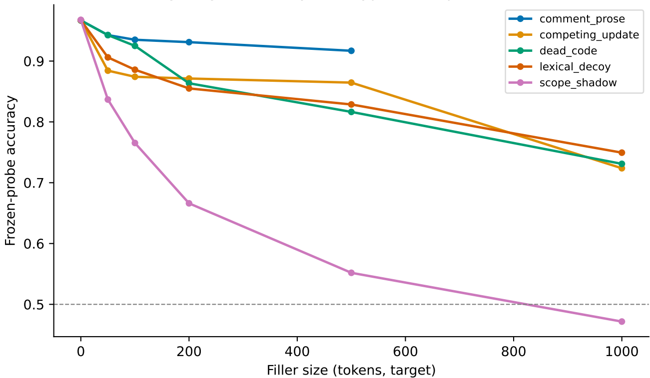
binding: degradation by filler type — deepseek-coder-1.3b
