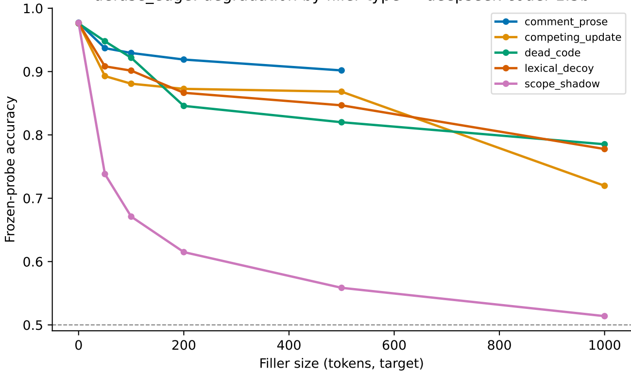
defuse_edge: degradation by filler type — deepseek-coder-1.3b
