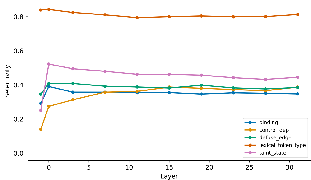
Probe selectivity by layer — deepseek-coder-6.7b_core
