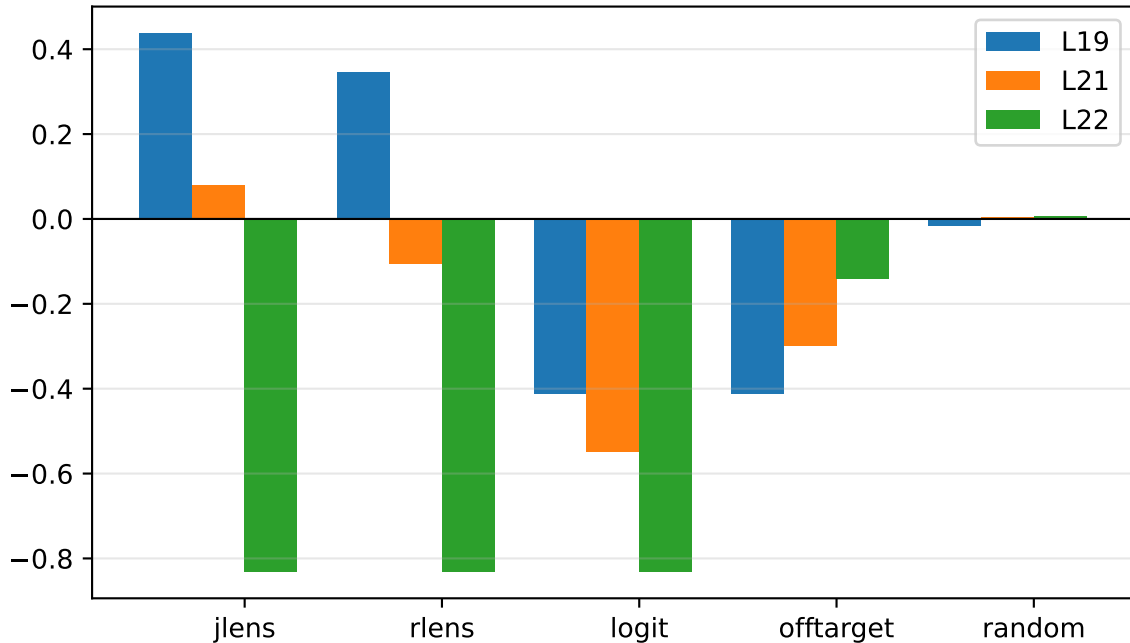
deepseek-coder-1.3b: erasing the lens read direction
