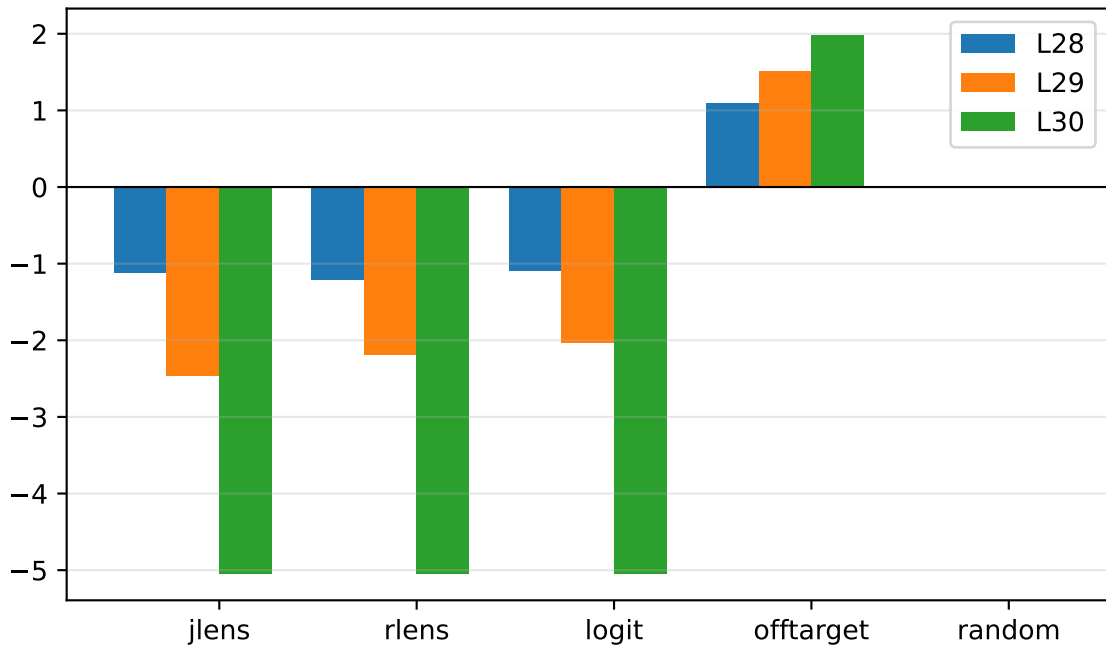
deepseek-coder-6.7b: erasing the lens read direction
