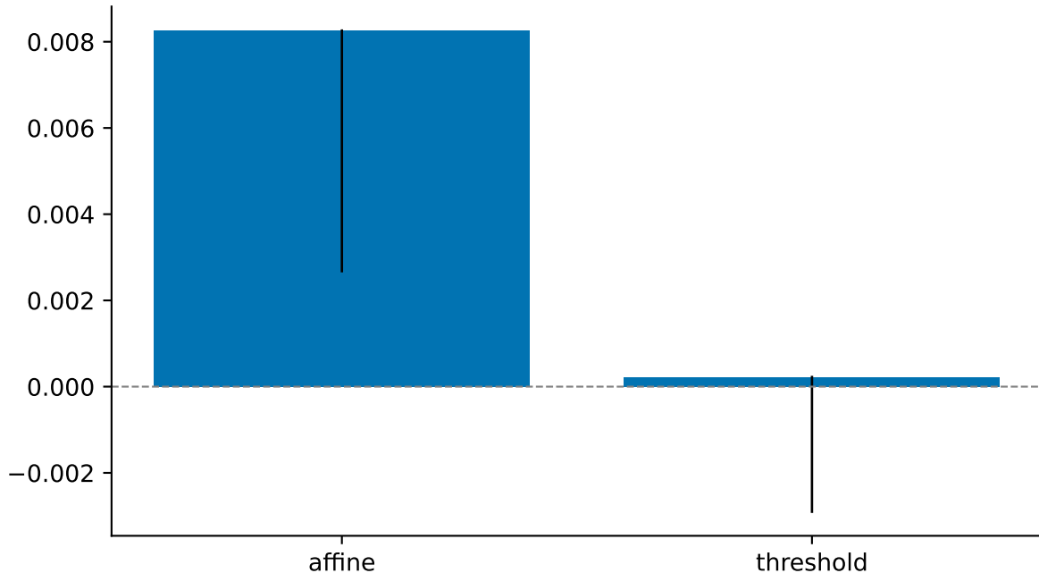
E11: one value swap, 2 downstream operations — deepseek-coder-1.3b (site L6+12+18, test split; bars below zero falsify the routing claim)
