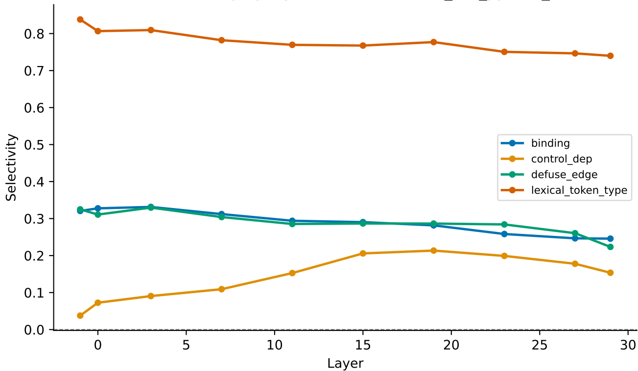
Probe selectivity by layer — starcoder2-3b_csn_python_200
