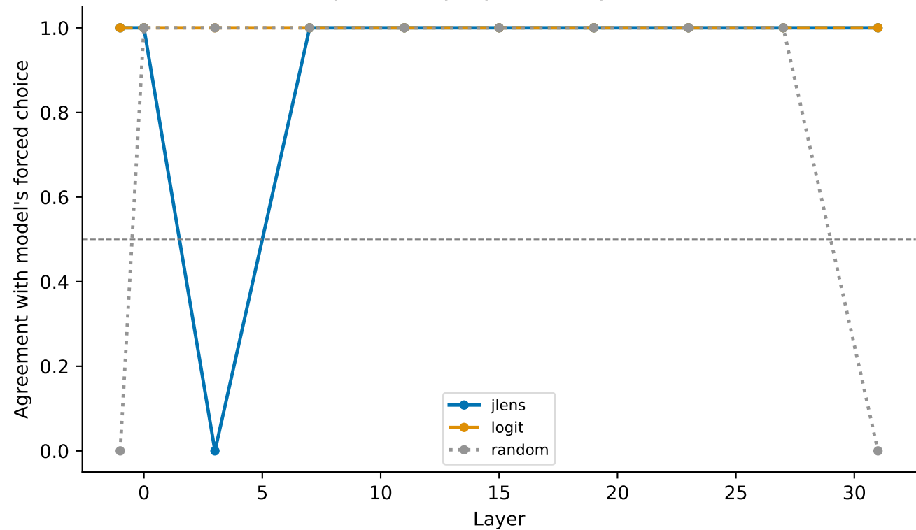
V3 taint disposition by layer — deepseek-coder-6.7b
