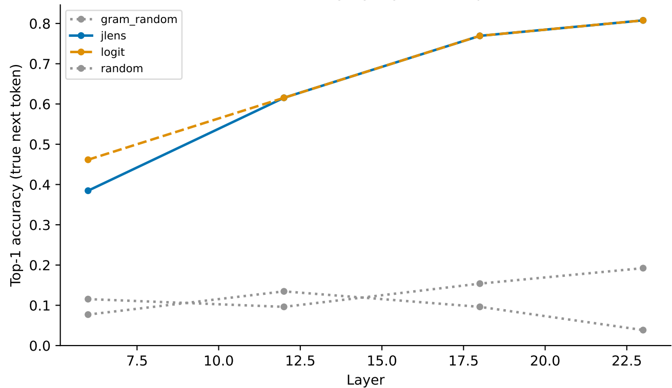
E11 V2: next-token recovery by layer — deepseek-coder-1.3b
