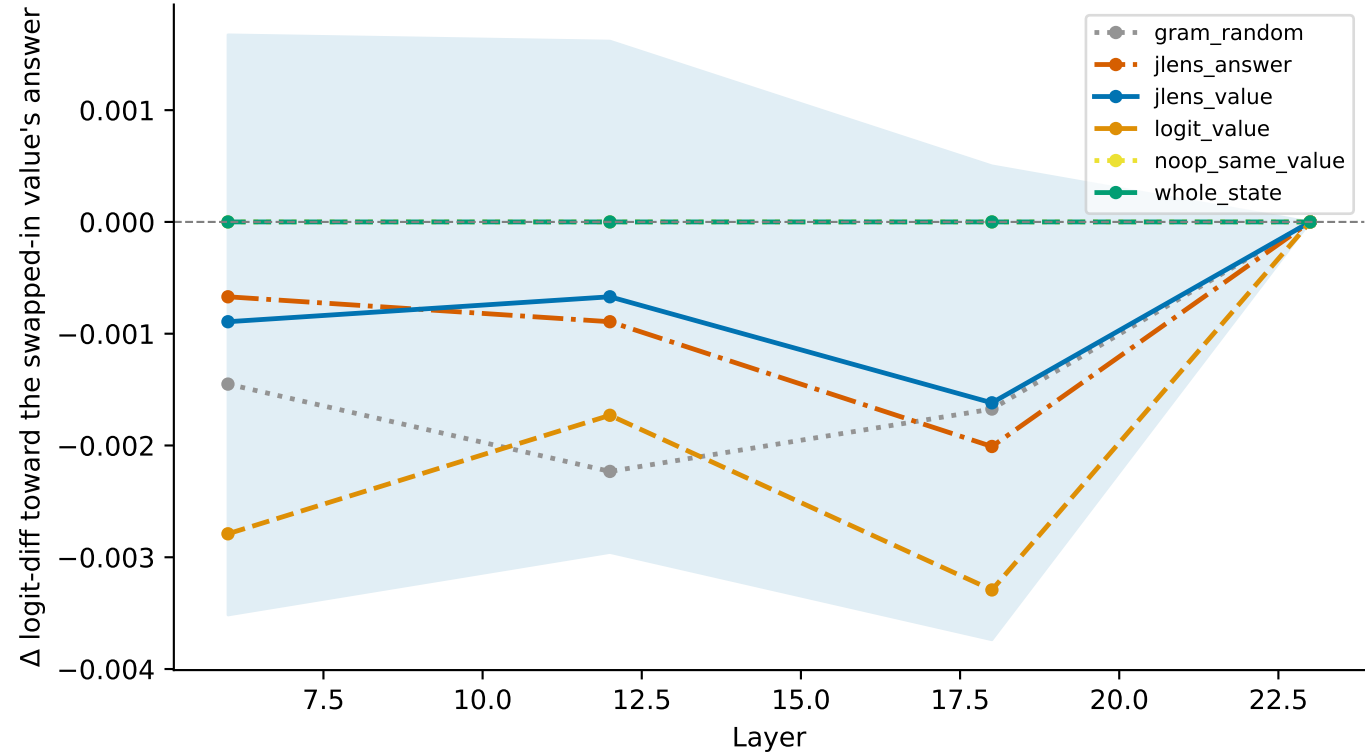
E11: J-space coordinate swap at the pre_def (control position) — deepseek-coder-1.3b
