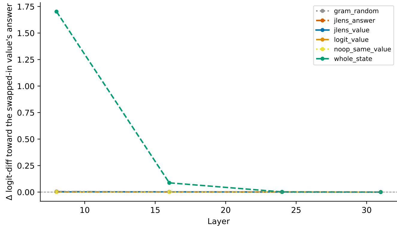
E11: J-space coordinate swap at the marked use — deepseek-coder-6.7b
