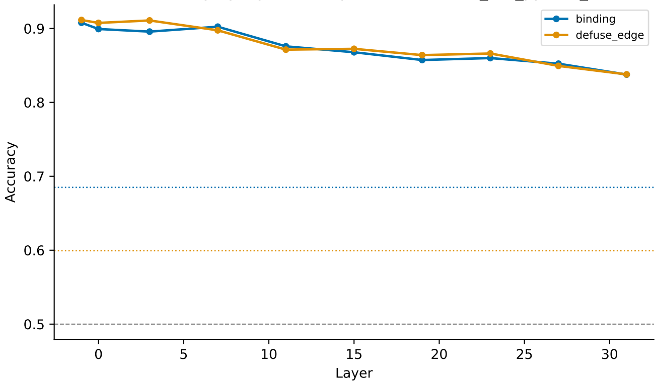
Probe accuracy by layer — deepseek-coder-6.7b_csn_python_200
