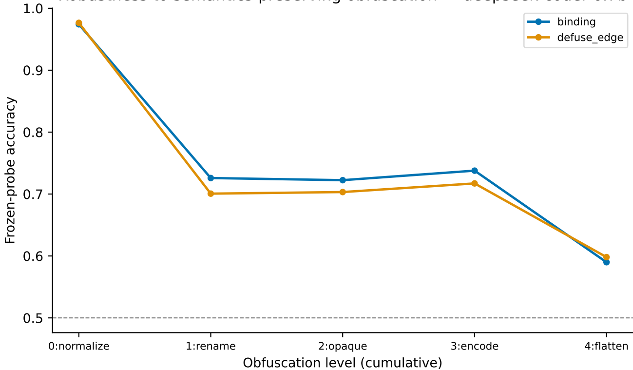
Robustness to semantics-preserving obfuscation — deepseek-coder-6.7b
