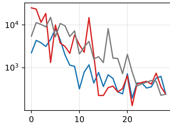
scopeword
