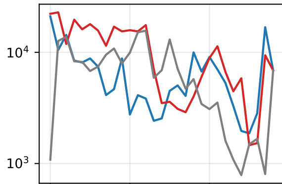
arith
