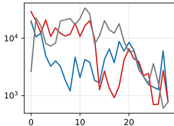
defuse
