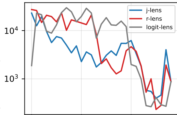
alias
