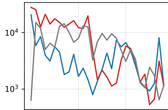
binding
