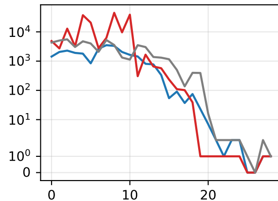
typeof
