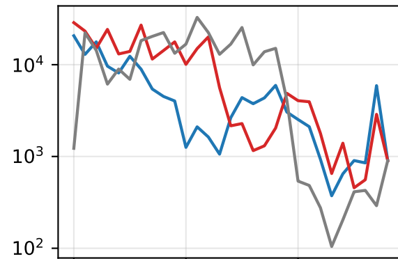
call
