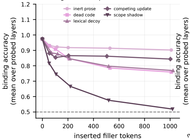
(a) Length is cheap, interference is not
