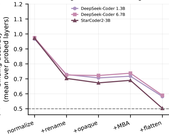
(b) Renaming survives, flattening does not
