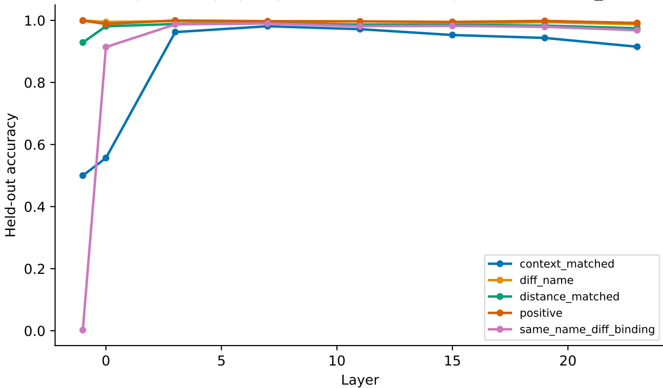
Binding accuracy by negative stratum — deepseek-coder-1.3b_core
