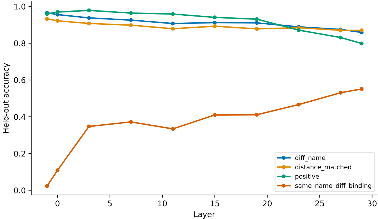
Binding accuracy by negative stratum — starcoder2-3b_csn_python_200
